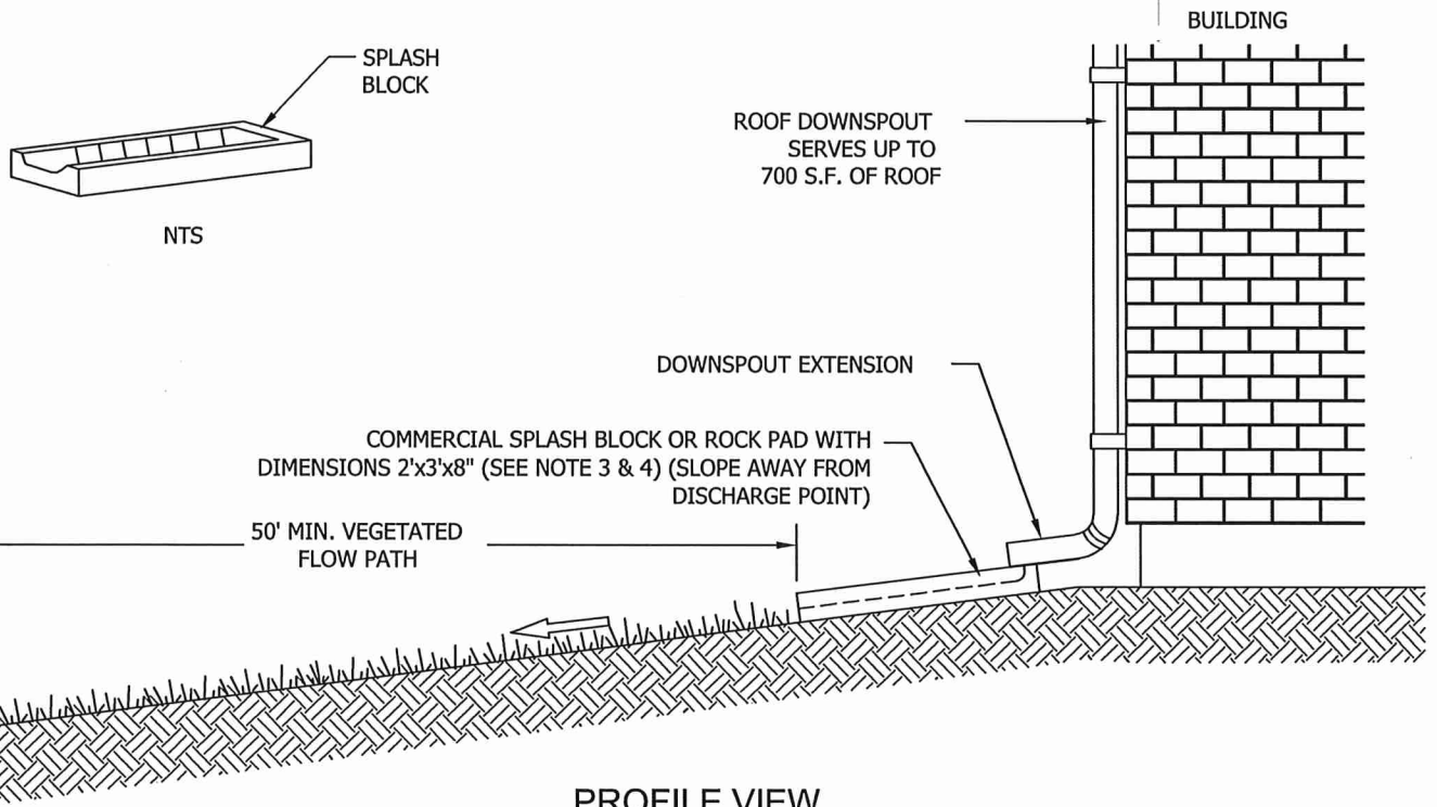
PROFILE VIEW
