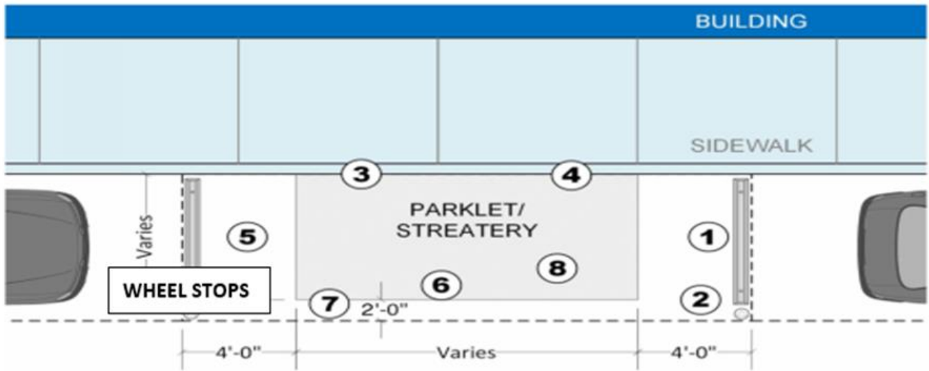
SINGLE SPACE PARKLET/CURBSIDE CAFÉ/MARKET FEATURES AND DIMENSIONS
